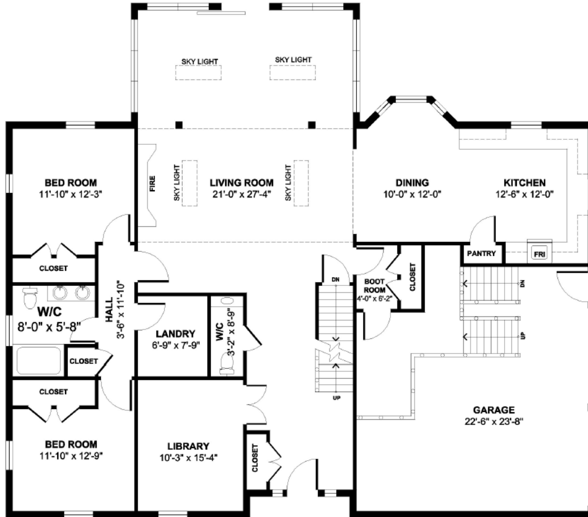
Main Floor 2270 square feet
